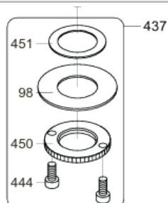
VR437 Vola Deck Spout Fixing Kit
